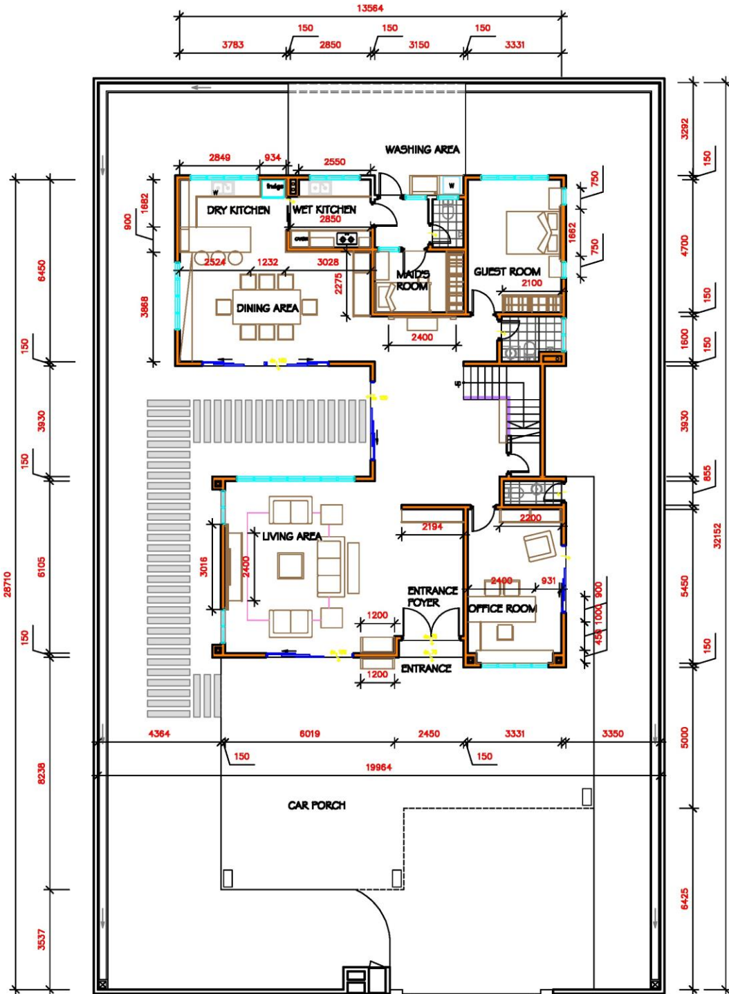
01 FURNITURE LAYOUT PLAN ( GROUND FLOOR ) ( BANGLO JENIS B )
